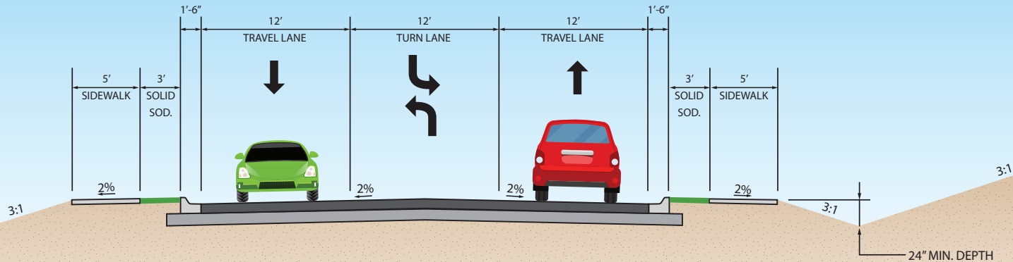
BYPASS URBAN TYPICAL SECTION – INITIAL
