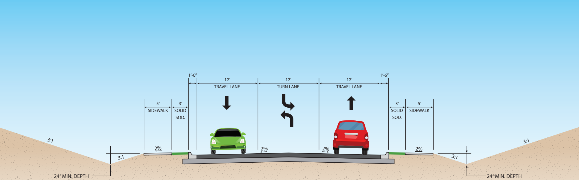
HIGHWAY 67 URBAN TYPICAL SECTION – INITIAL
